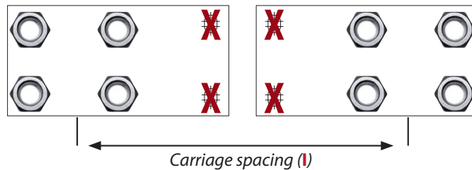
Using the CG-05P foundation plate with CGS / CGA "M" carriages
