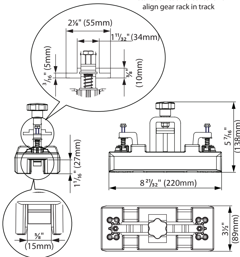
The Integrator Gear Rack Installation Tool
